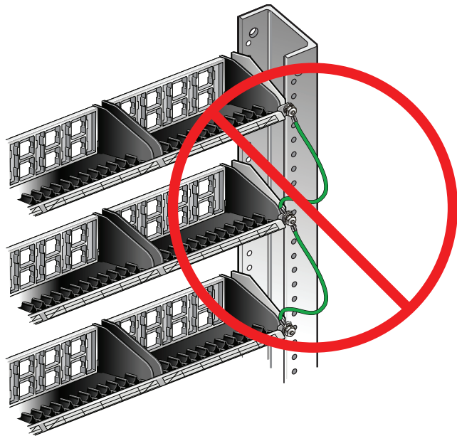
Figure 3: Daisy Chaining of Ground Straps is Not Allowed.
