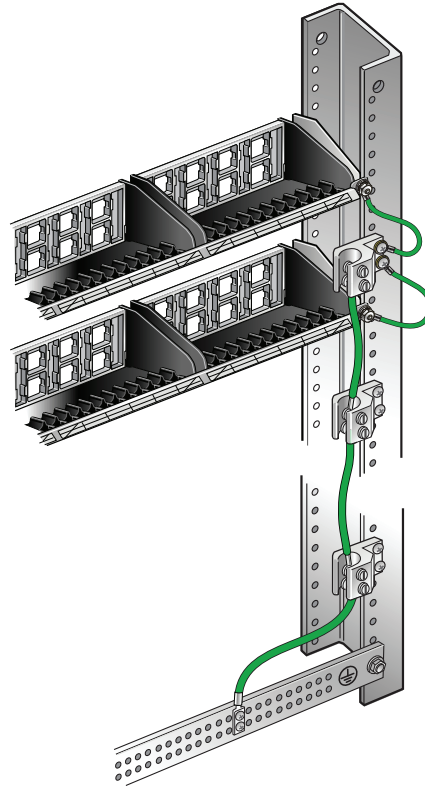
Figure 5: Panels Grounded to Earthing Terminals, Then to the Telecommunications Grounding Bus-Bar
