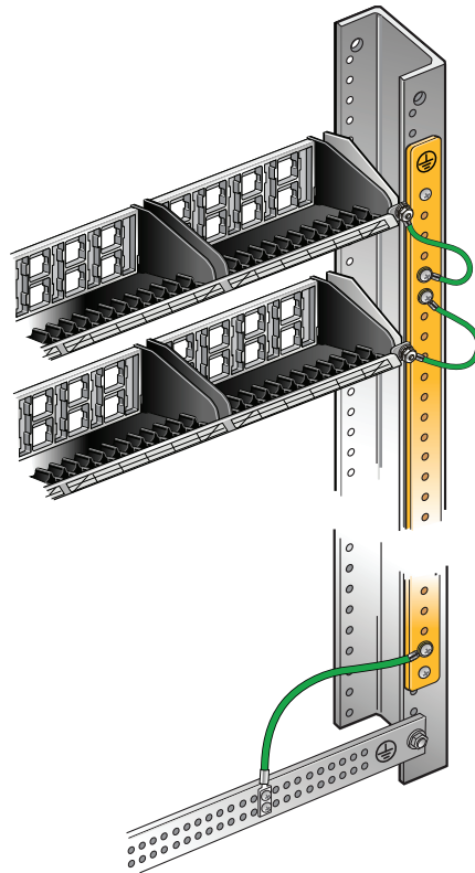
Figure 4: Use of Vertical Grounding Bus-Bar
