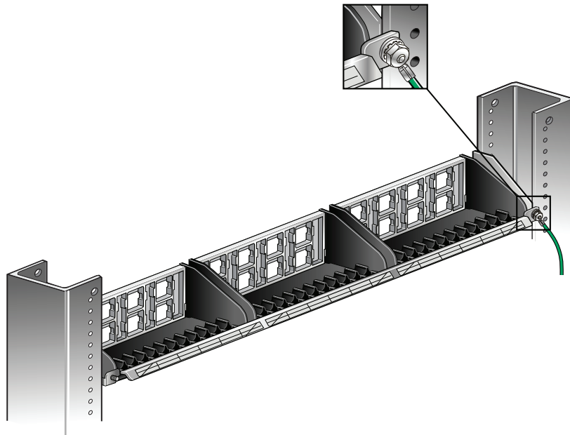
Figure 1: Connecting the Ground Strap to the Earthing Stud on the Back of the Panel
