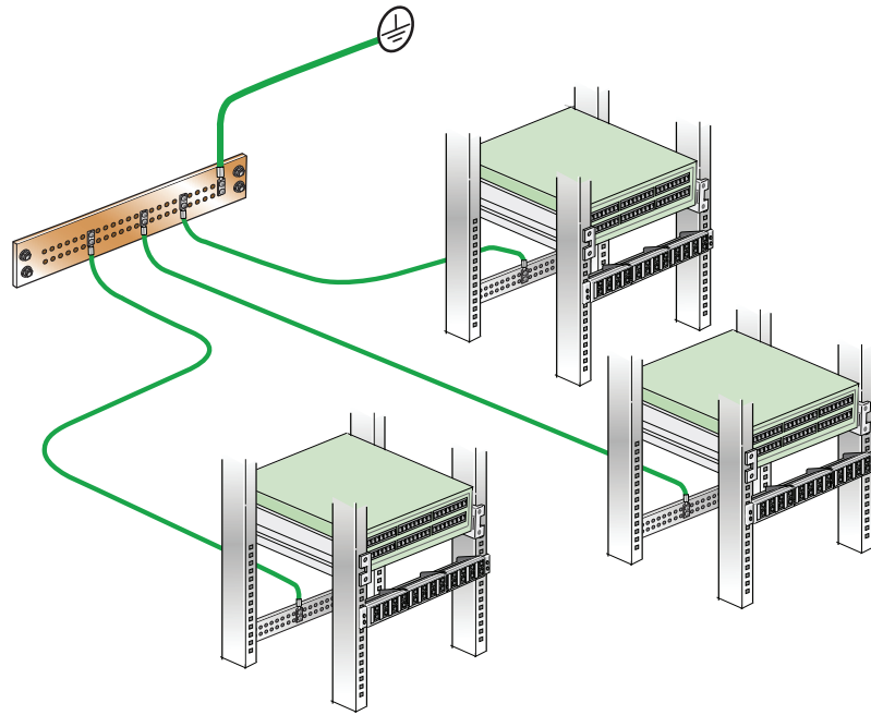
Figure 6: Earthing and Bonding of Equipment Cabinets/Racks
