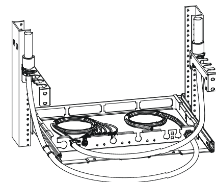
InstaPATCH Plus Attachment Bracket
