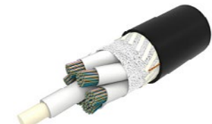
Indoor/Outdoor Rollable Ribbon Loose Tube Cable
